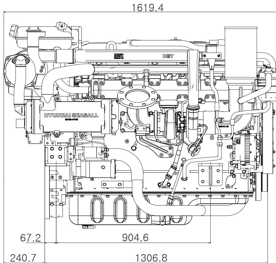
Side View
